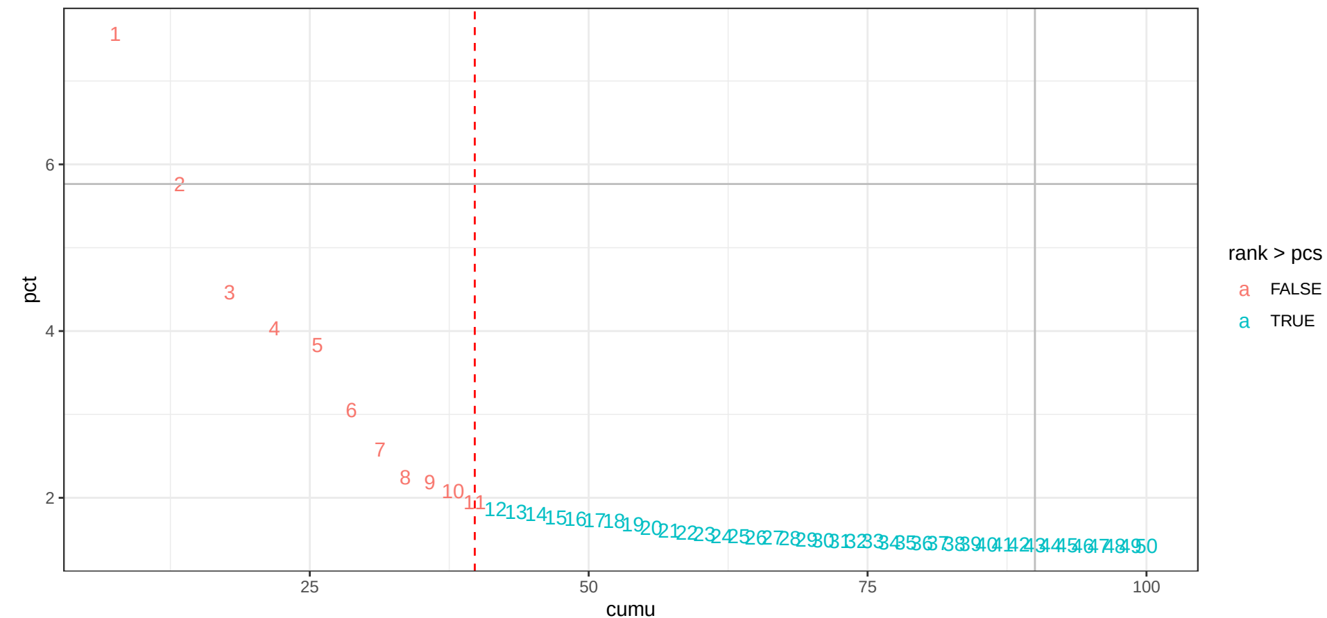
Elbow Plot – Selected PCs: 11
